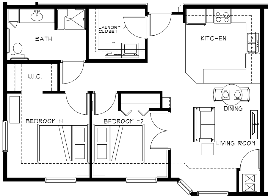
GOODHUE TYPE "B" 905 S.F. 2 BEDROOM (2) TOTAL (2) w/ DECK (1) DELUXE UNIT
