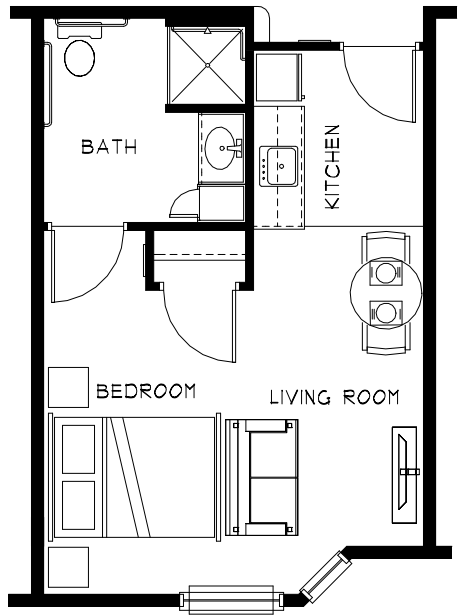
LEGACY A.1 TYPE "B" 385 S.F. STUDIO (2) TOTAL
