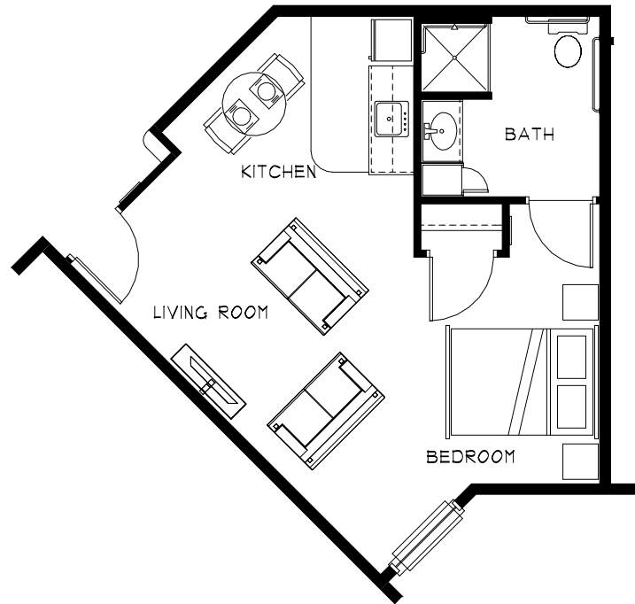
LEGACY A.4 TYPE "B" 481 S.F. STUDIO (1) TOTAL
