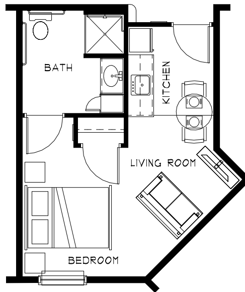
LEGACY A.5 TYPE "B" 349 S.F. STUDIO (1) TOTAL
